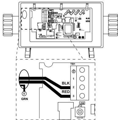
Figure C Connections (North American 60 Hz 240 VAC 3-Wire Connection Models)
